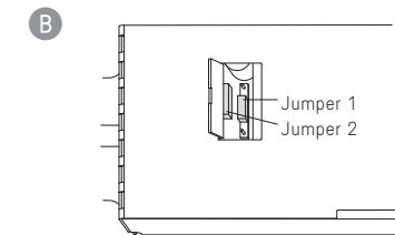
Setting for 230 V / 50–60 Hz (Second jumper mounted under cover housing)
