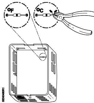
Figure 3. Jumper Location.
