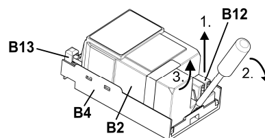
figure 8: dismounting an RL module
