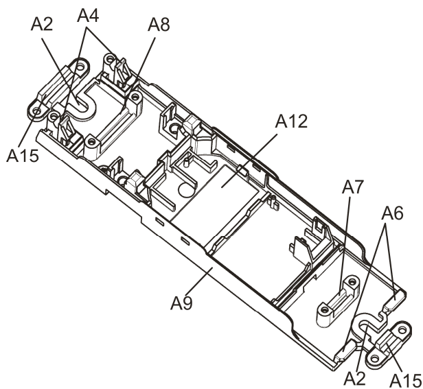
figure 2b: Mounting
