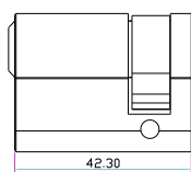
Single side cylinde
